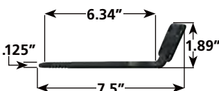
Wall Bracket
