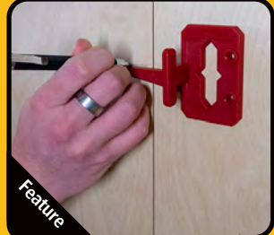
Marking centerline for hinge cup
